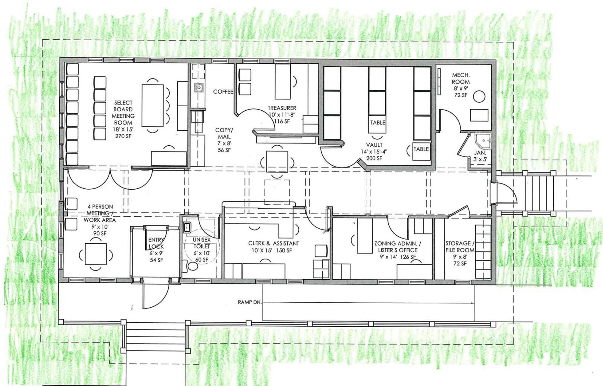
PROPOSED FLOOR PLAN 1984 GSF
